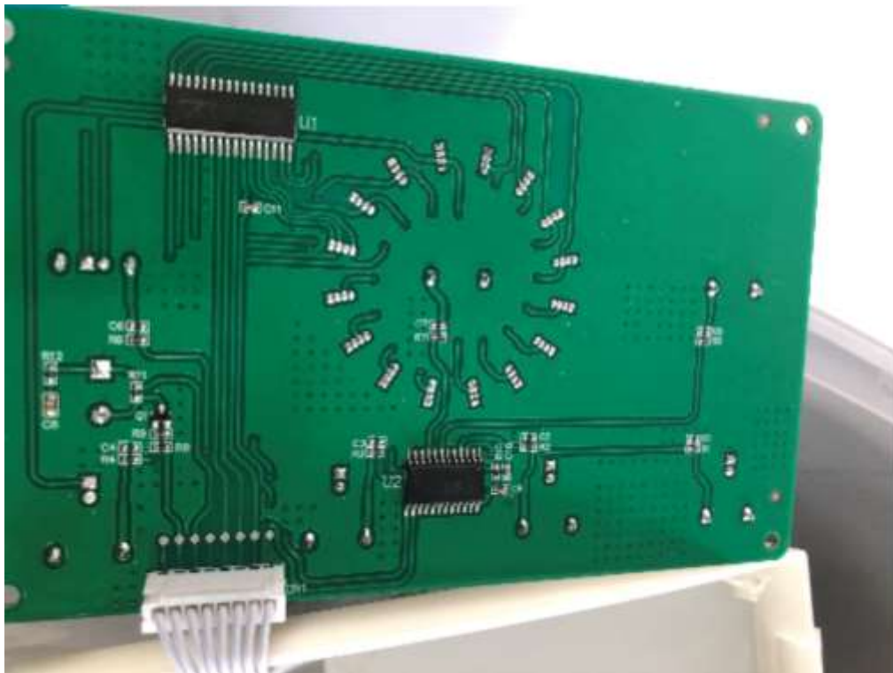
Fig. 17 PCB 2 view for all models
